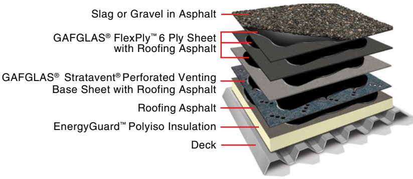
TYPICAL 4-PLY PREMIUM SYSTEM WITH GAFGLAS® STRATAVENT®, FLEXPLY™ 6, FLOOD COAT, AND GRAVEL
